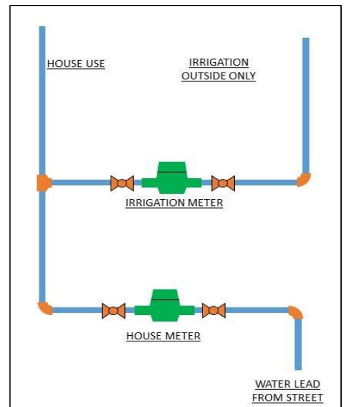
Irrigation Meter Diagram
