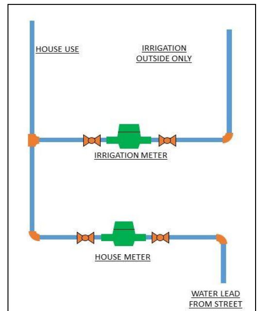
Irrigation Meter Diagram
